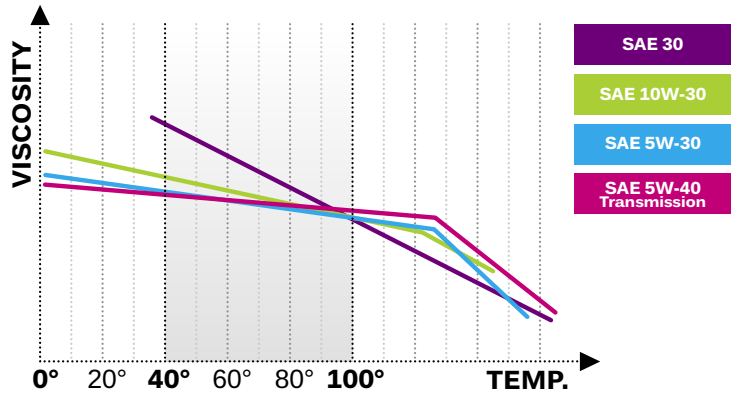
Viscosity performance
